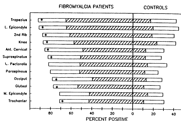
Figure 1. Percentage of fibromyalgia patients and control patients with "mild or greater" or "moderate or greater" tenderness at the 24 tender point sites examined. Values are means of the paired (left and right) tender point sites. Open bars show mild or greater tenderness; hatched bars show moderate or greater tenderness. * = tender point site retained in the 1990 criteria for fibromyalgia. L = left; Ant. = anterior; M. = medial.
