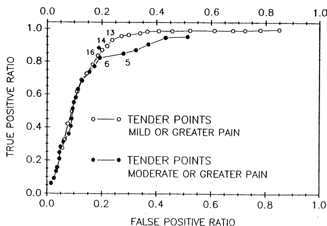
Figure 2. Empiric receiver operating characteristic curves for cumulative number of tender point sites scored either as mild or greater tenderness or as moderate or greater tenderness. Twenty-four "active" sites were examined. True positive ratio = the proportion of patients with fibromyalgia at each tender point score; false positive ratio = the proportion of controls at each tender point score. ♦ = sensitivity and specificity of 1990 criteria (11 of 18 tender points and widespread pain).
